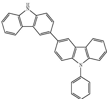
Chemical Formula 8
