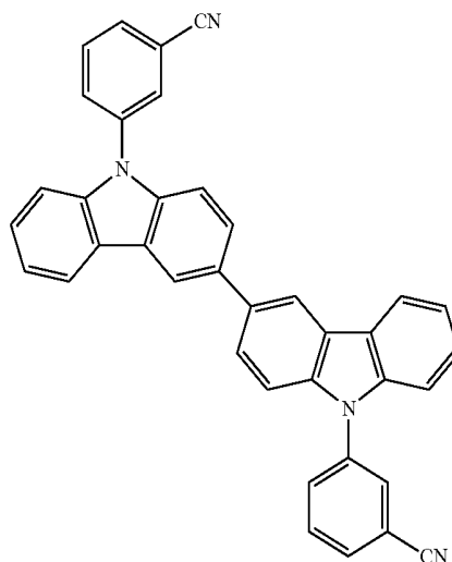
Chemical Formula 9
