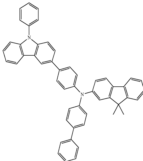
Chemical Formula 3
