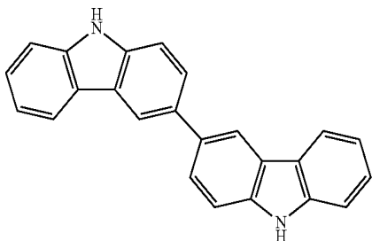
Chemical Formula 5
