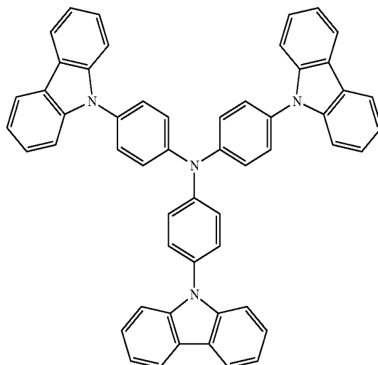
Chemical Formula 3
